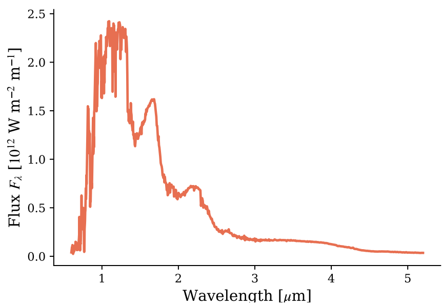
Disk
