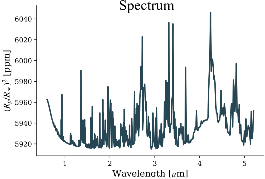
Disk + Transit
