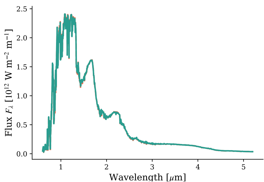
Stellar Spectrum
