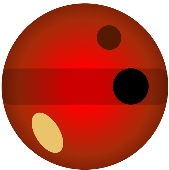
Transit
