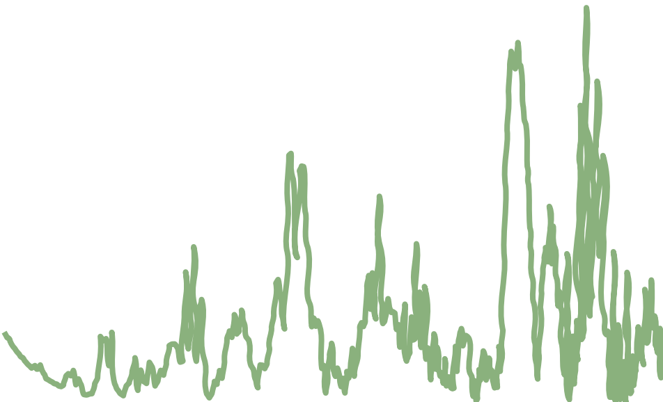
Reconstructed Spectrum
