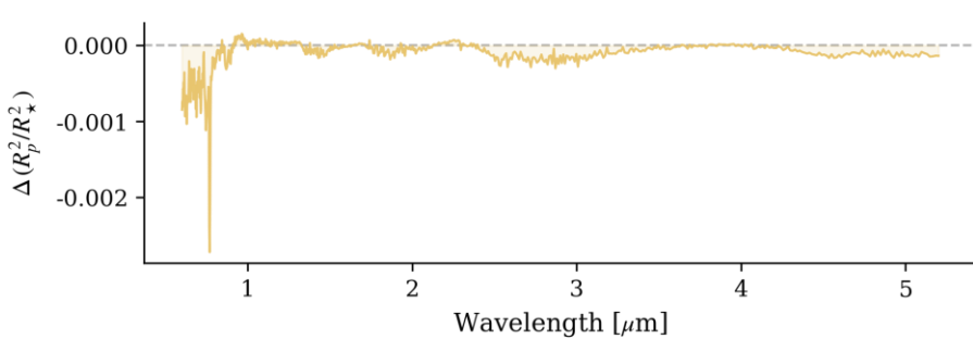
Residuals
