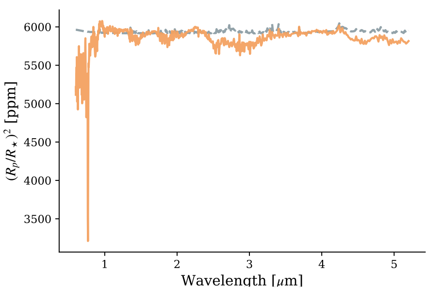
Transit
